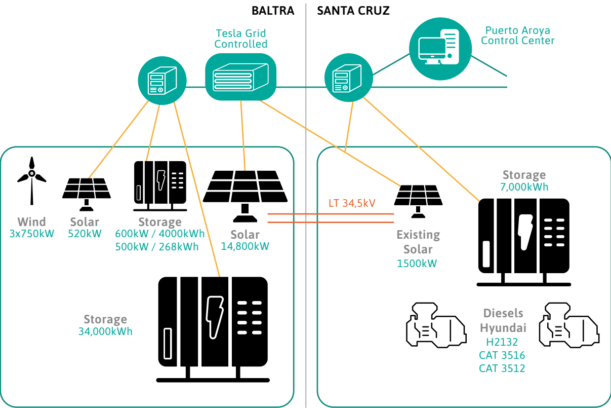
SYSTEM LEVEL VIEW OF SOLUTION FOR SANTA CRUZ AND BALTRA
